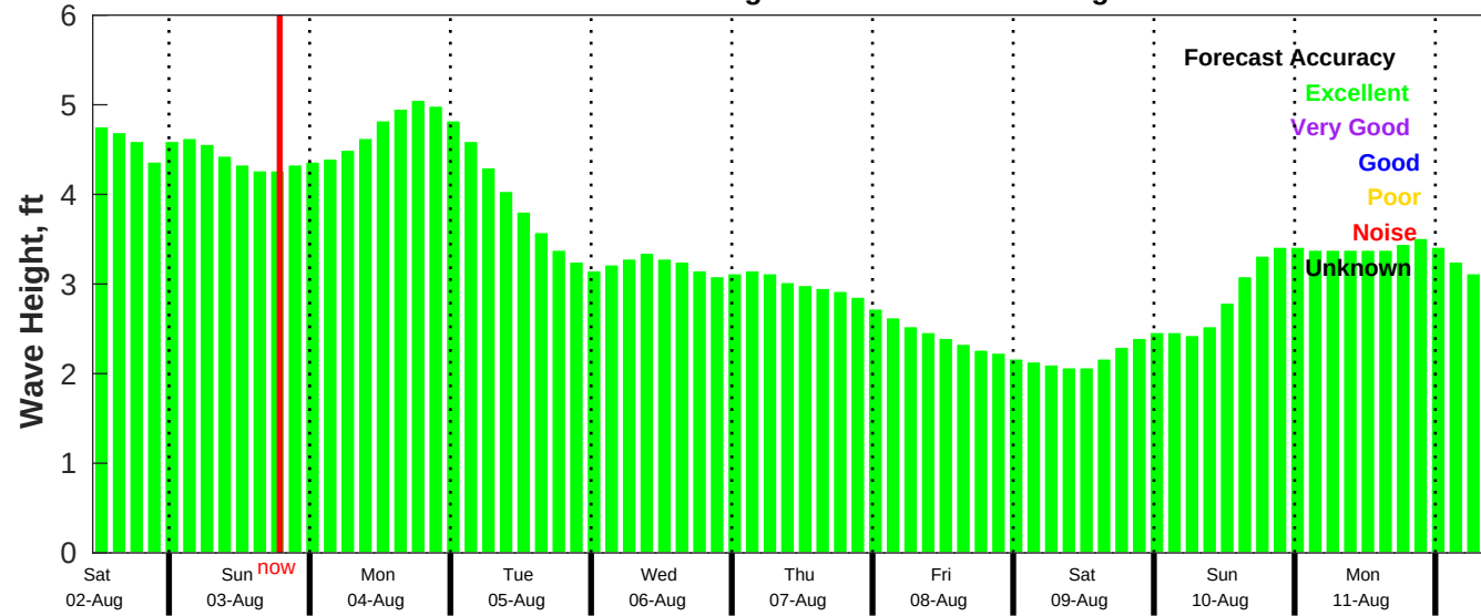
CMEMS Wave Forecast for NDBC 52211 from 01-Aug-2025 11:00:00 to 11-Aug-2025 11:00:00
