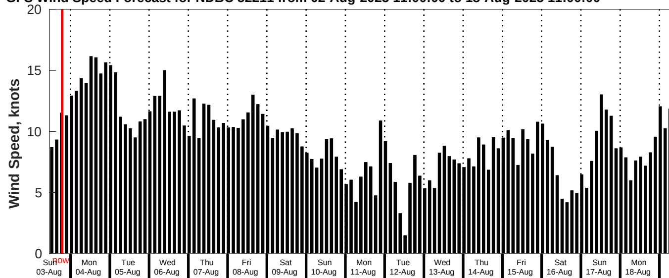
GFS Wind Speed Forecast for NDBC 52211 from 02-Aug-2025 11:00:00 to 18-Aug-2025 11:00:00
