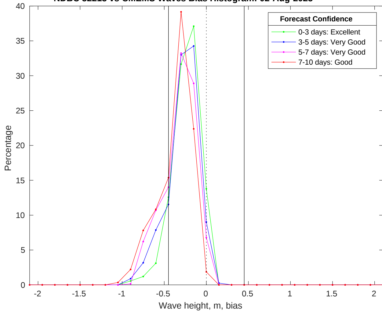
NDBC 52213 vs CMEMS Waves Bias Histogram: 02-Aug-2025
