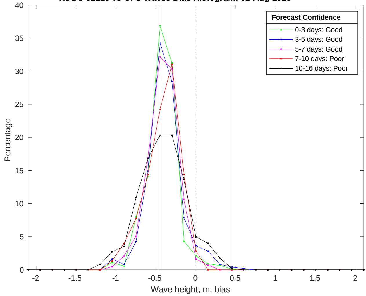
NDBC 52213 vs GFS Waves Bias Histogram: 02-Aug-2025
