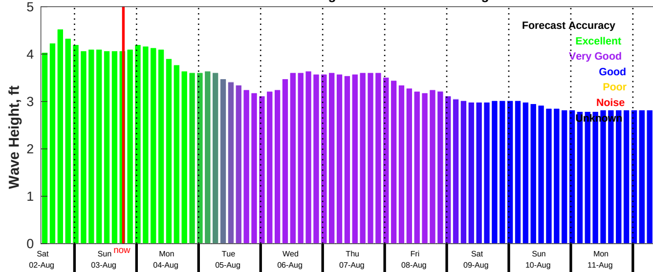
CMEMS Wave Forecast for NDBC 52213 from 01-Aug-2025 11:00:00 to 11-Aug-2025 11:00:00
