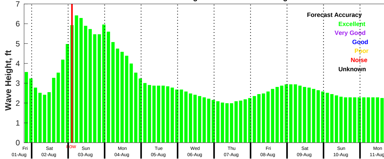
CMEMS Wave Forecast for NDBC 41004 from 01-Aug-2025 19:00:00 to 11-Aug-2025 19:00:00
