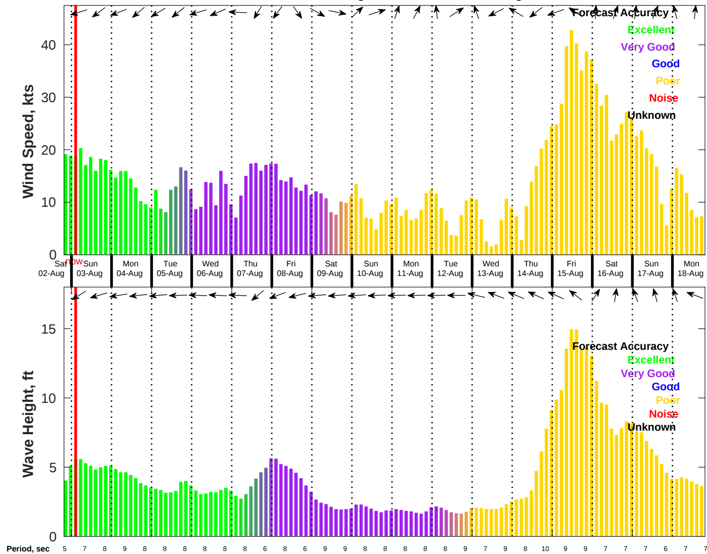
Wind & Wave Forecast for NDBC 41004 from 02-Aug-2025 19:00:00 to 18-Aug-2025 19:00:00
