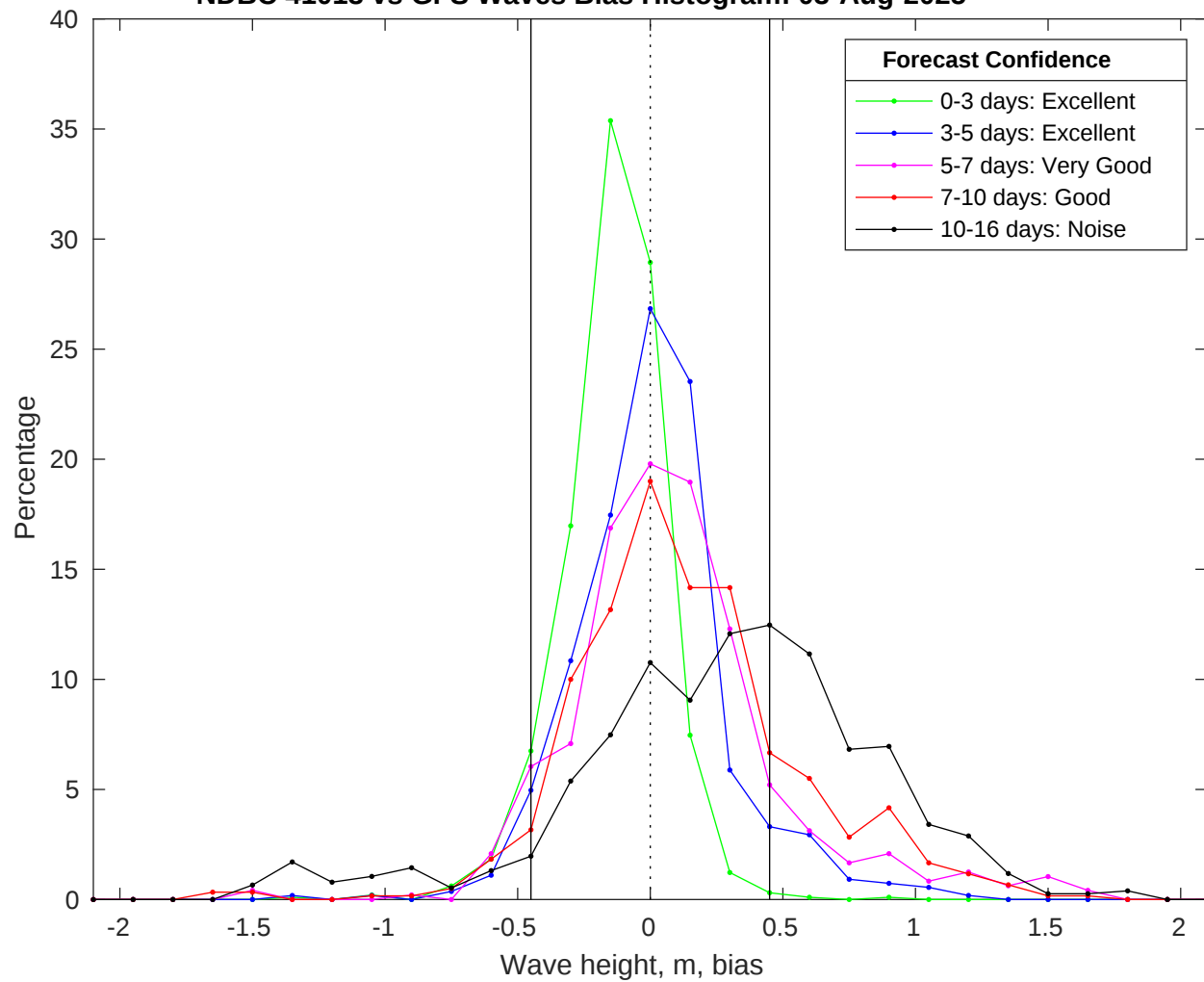
NDBC 41013 vs GFS Waves Bias Histogram: 03-Aug-2025
