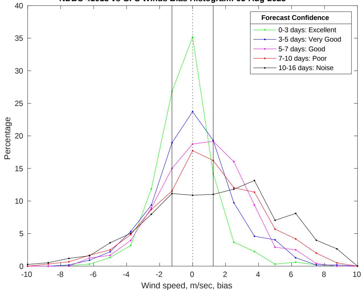
NDBC 41013 vs GFS Winds Bias Histogram: 03-Aug-2025
