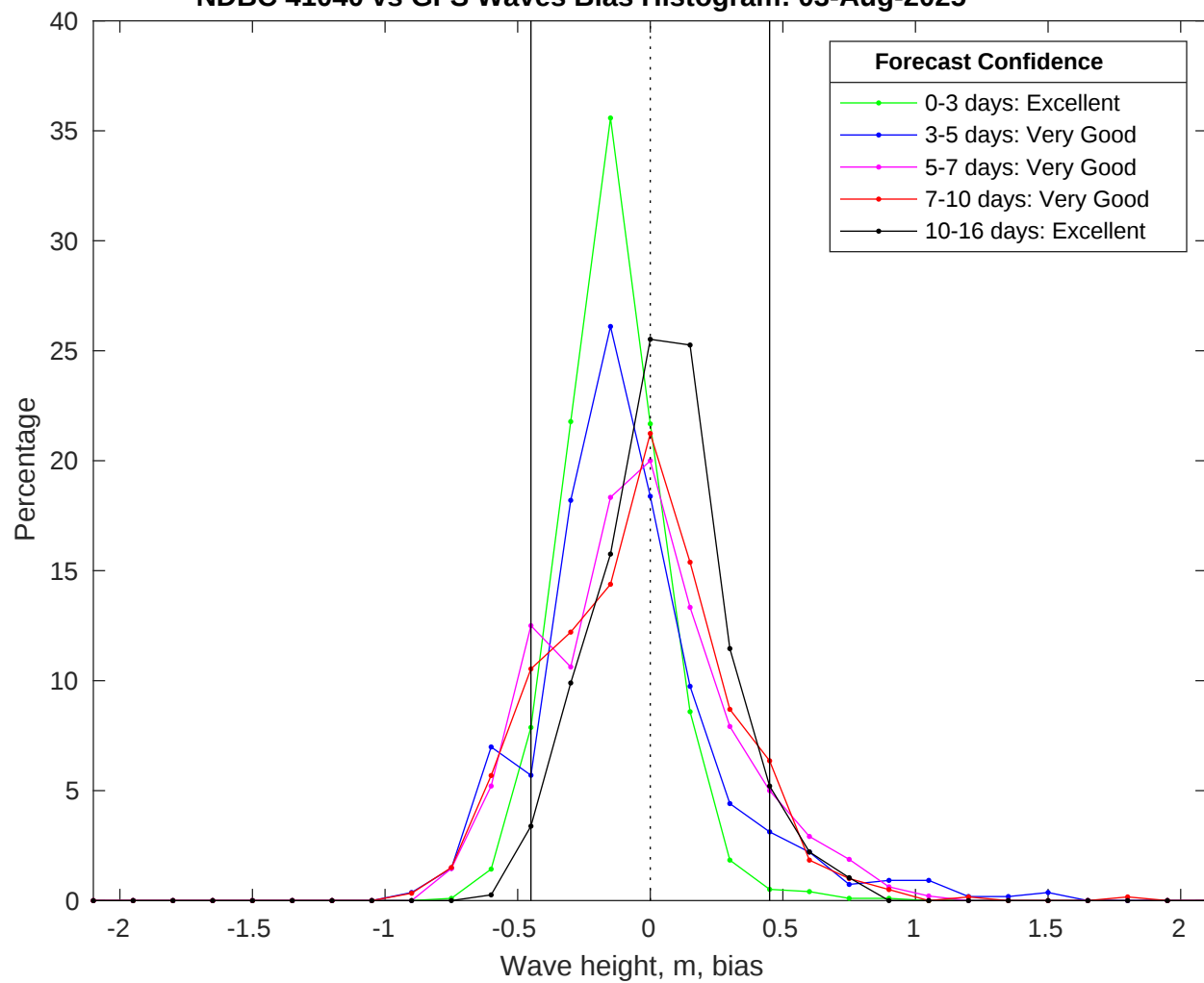
NDBC 41040 vs GFS Waves Bias Histogram: 03-Aug-2025
