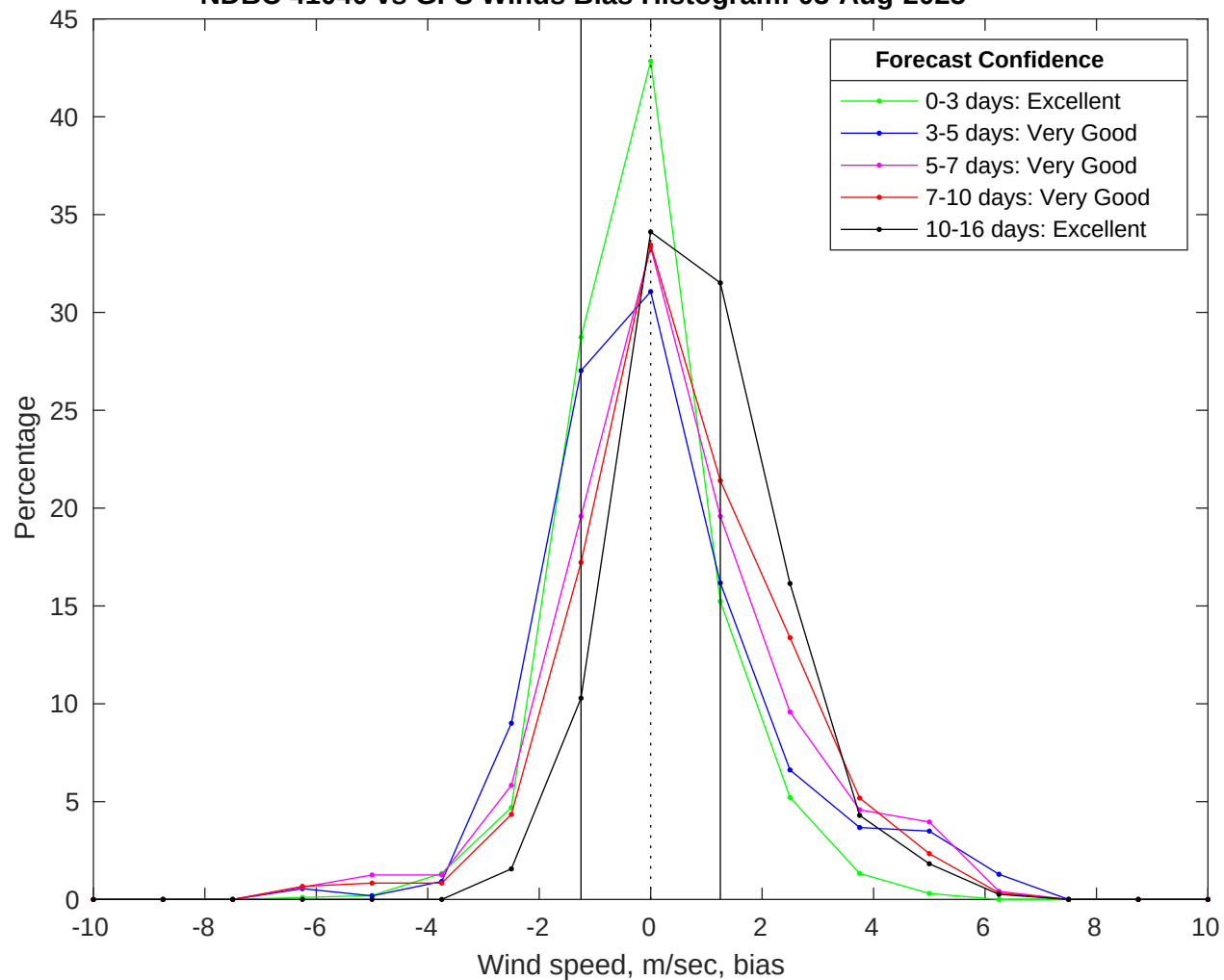
NDBC 41040 vs GFS Winds Bias Histogram: 03-Aug-2025
