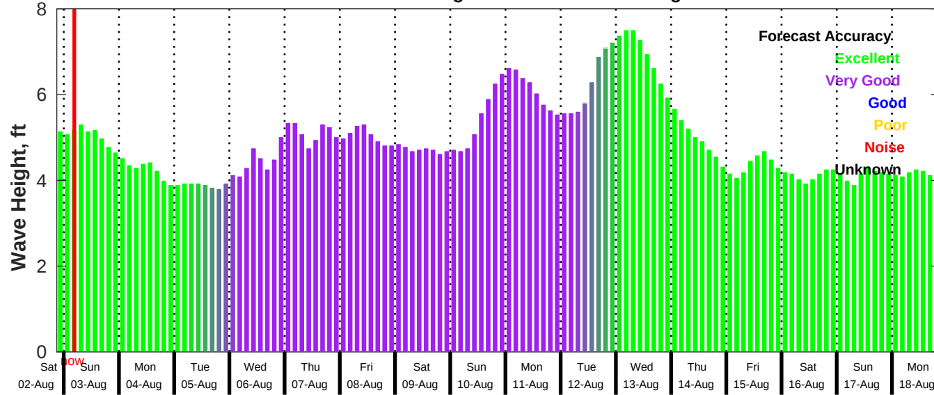
GFS Wave Forecast for NDBC 41040 from 02-Aug-2025 21:00:00 to 18-Aug-2025 21:00:00
