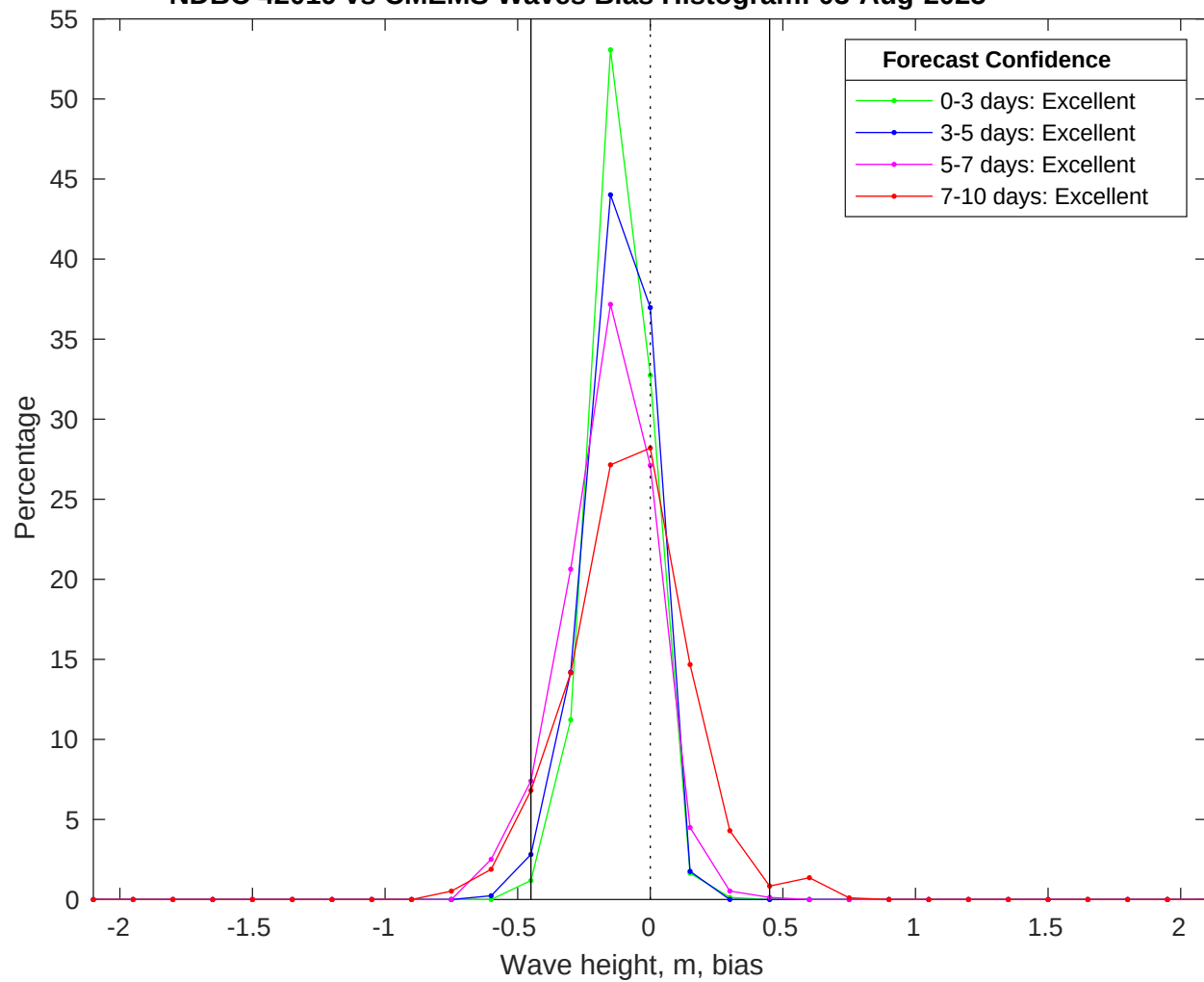
NDBC 42019 vs CMEMS Waves Bias Histogram: 03-Aug-2025
