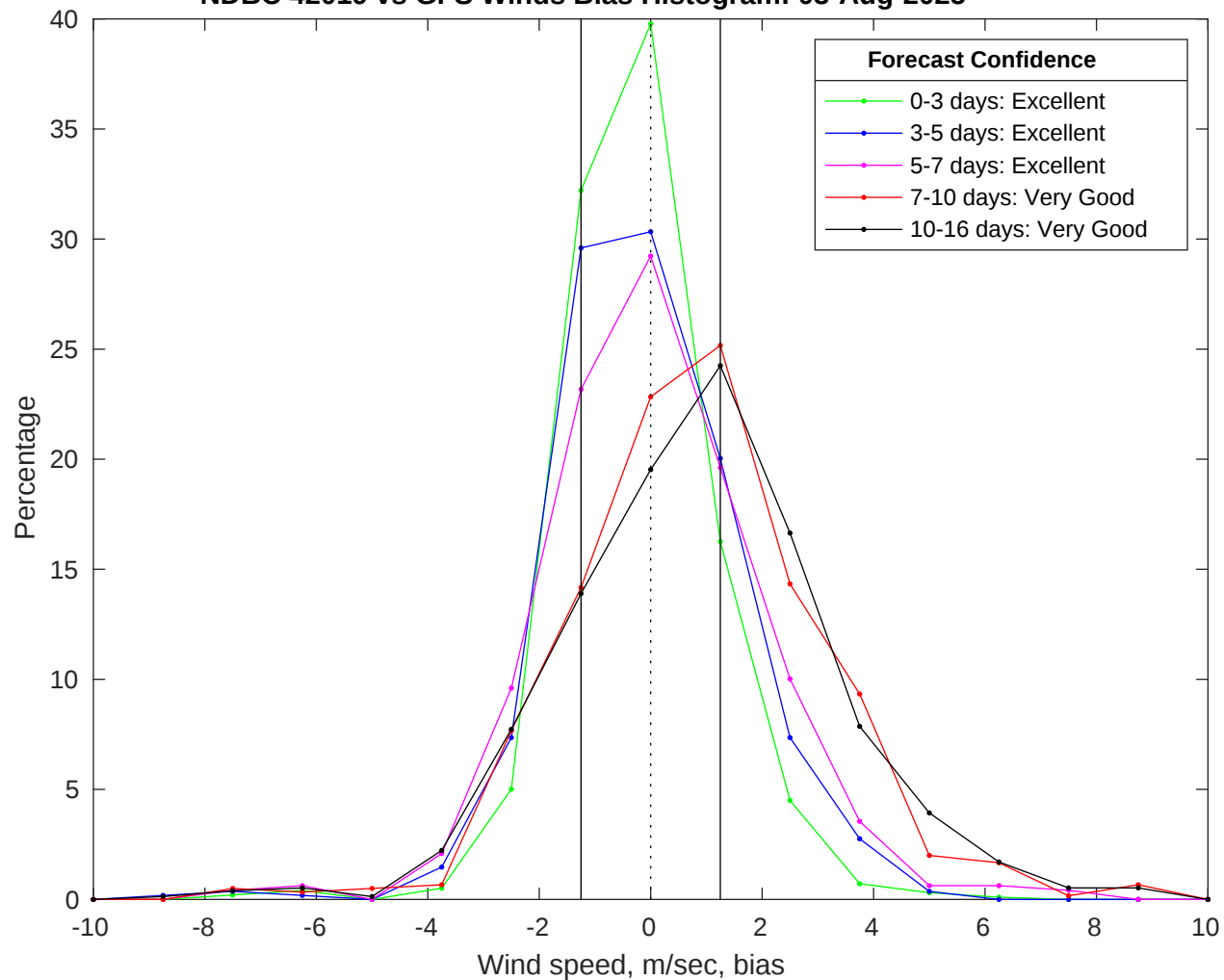
NDBC 42019 vs GFS Winds Bias Histogram: 03-Aug-2025
