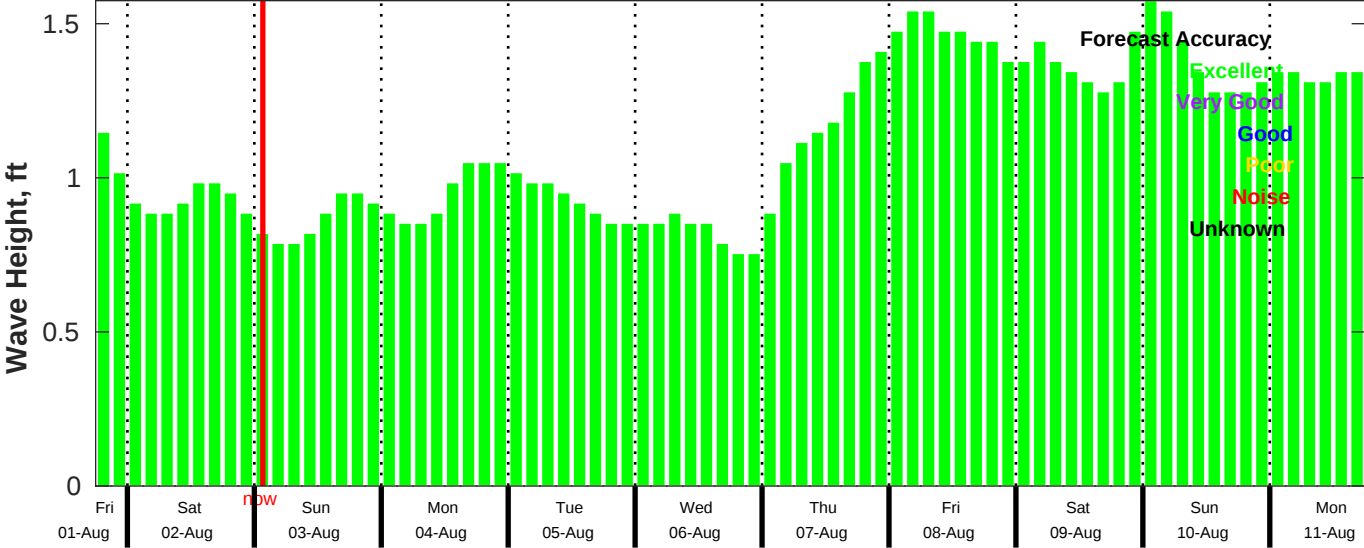
CMEMS Wave Forecast for NDBC 42019 from 01-Aug-2025 18:00:00 to 11-Aug-2025 18:00:00
