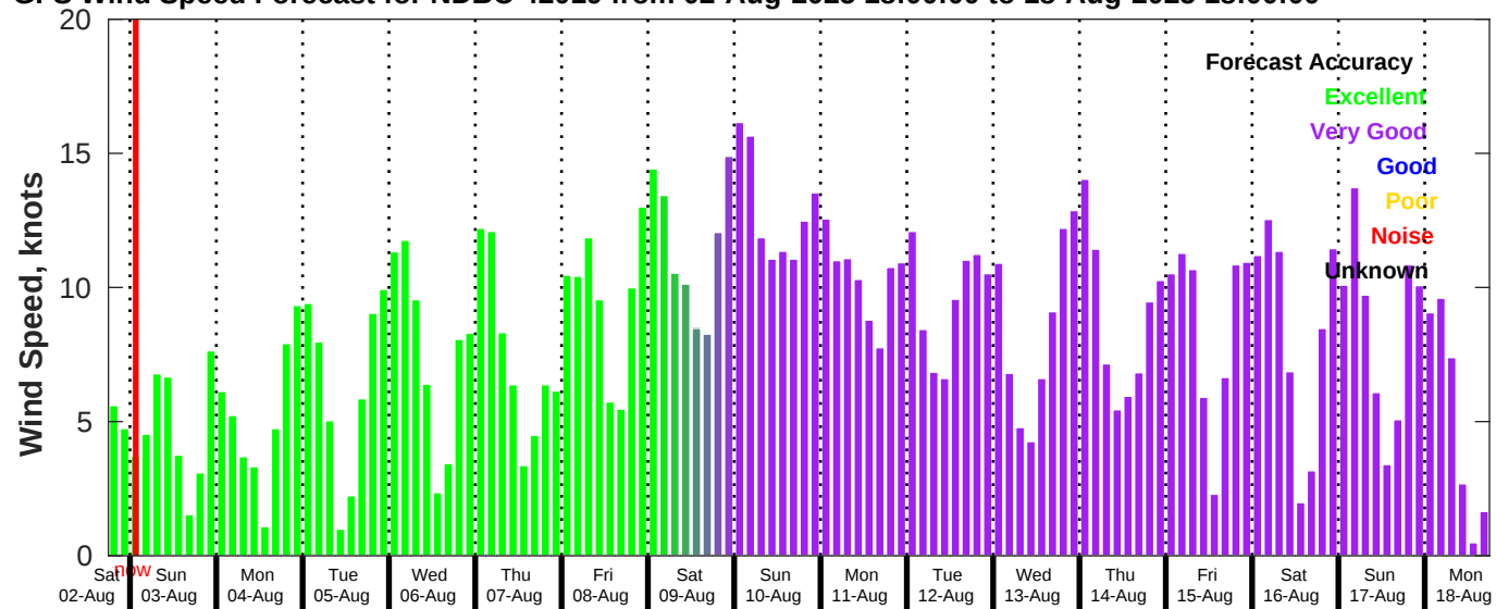
GFS Wind Speed Forecast for NDBC 42019 from 02-Aug-2025 18:00:00 to 18-Aug-2025 18:00:00
