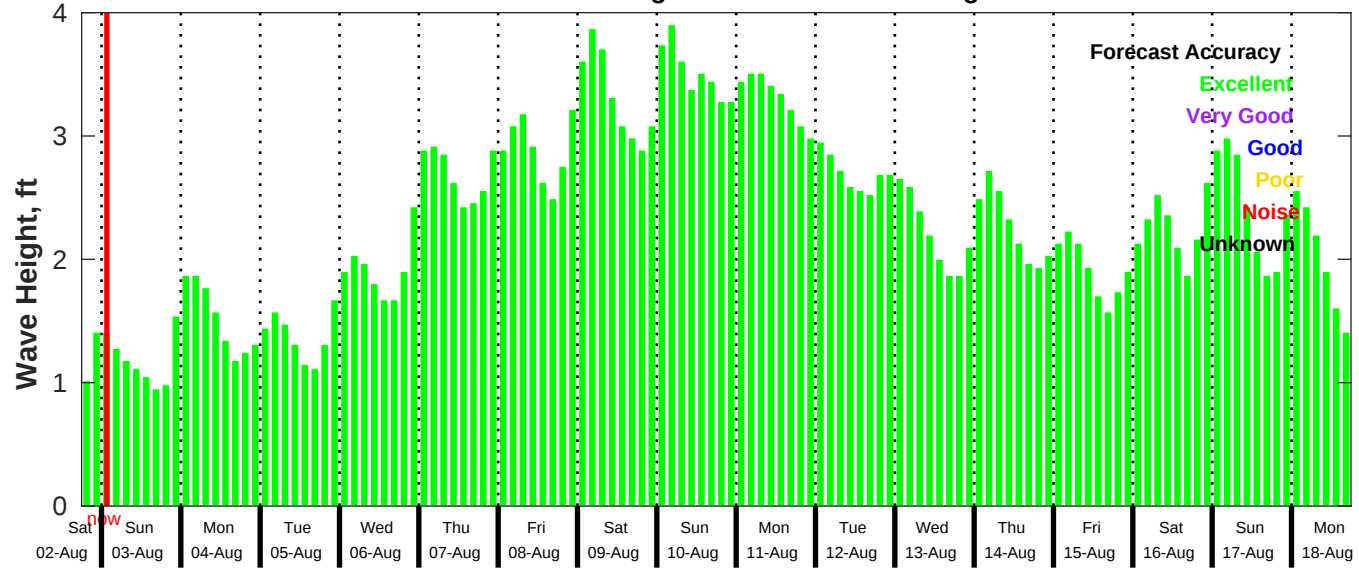
GFS Wave Forecast for NDBC 42020 from 02-Aug-2025 18:00:00 to 18-Aug-2025 18:00:00
