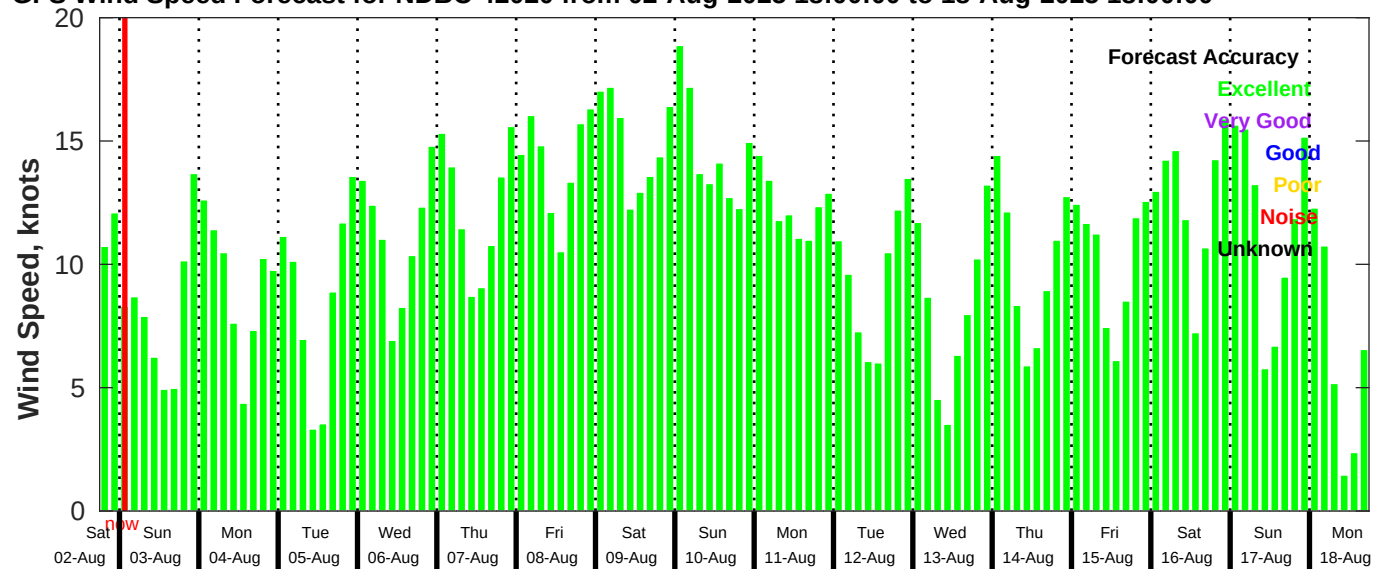
GFS Wind Speed Forecast for NDBC 42020 from 02-Aug-2025 18:00:00 to 18-Aug-2025 18:00:00
