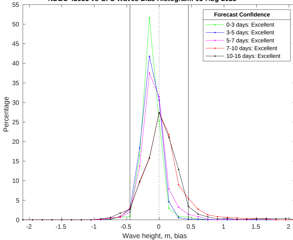
NDBC 42035 vs GFS Waves Bias Histogram: 03-Aug-2025
