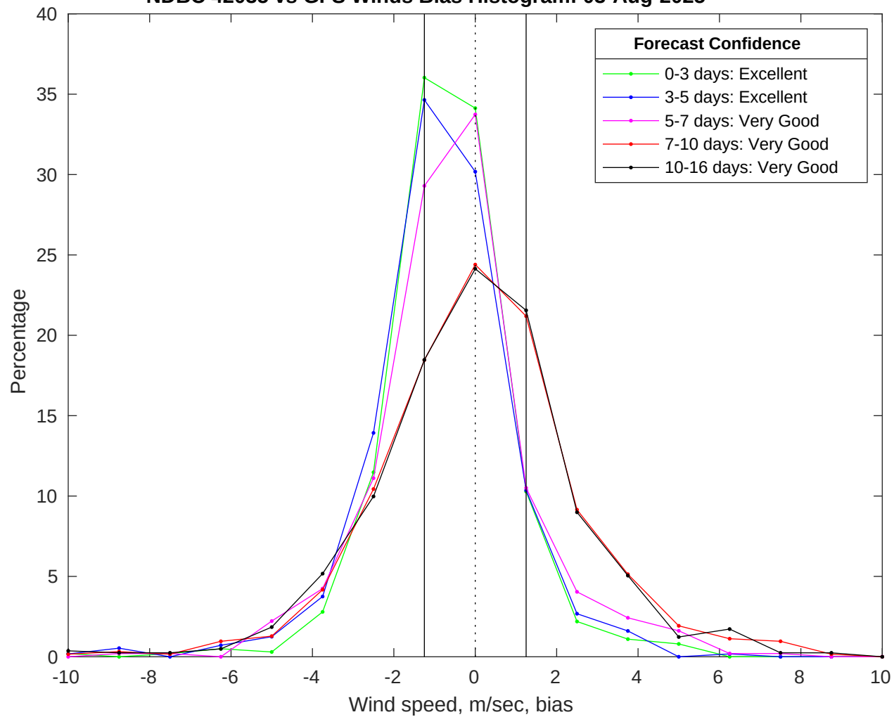
NDBC 42035 vs GFS Winds Bias Histogram: 03-Aug-2025
