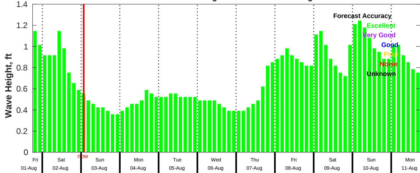
CMEMS Wave Forecast for NDBC 42035 from 01-Aug-2025 18:00:00 to 11-Aug-2025 18:00:00
