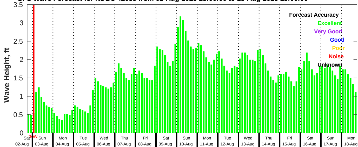
GFS Wave Forecast for NDBC 42035 from 02-Aug-2025 18:00:00 to 18-Aug-2025 18:00:00
