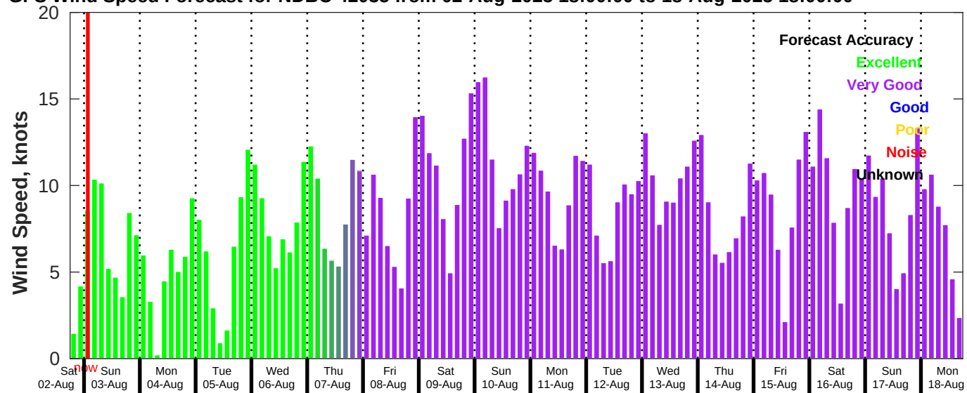
GFS Wind Speed Forecast for NDBC 42035 from 02-Aug-2025 18:00:00 to 18-Aug-2025 18:00:00
