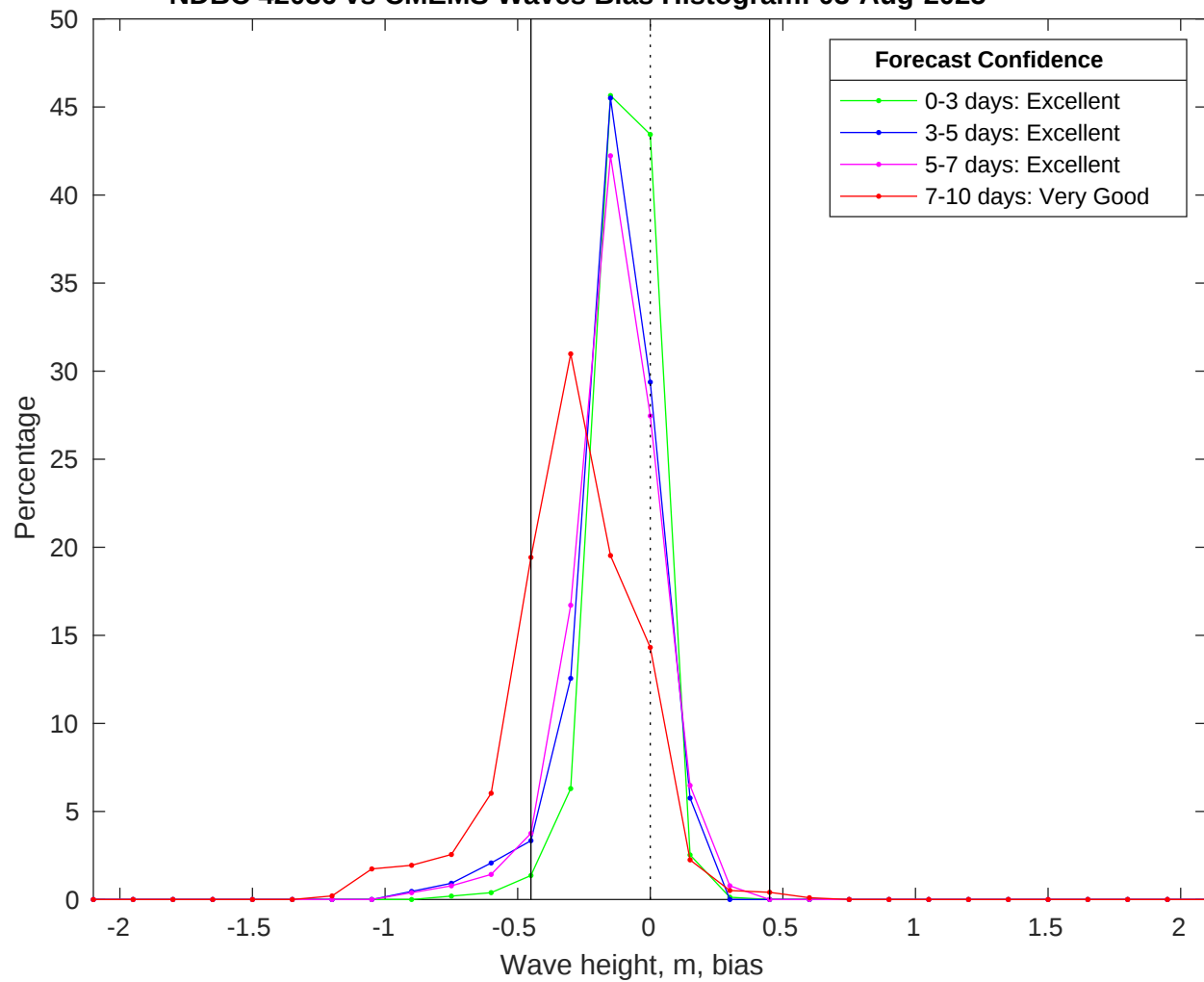
NDBC 42036 vs CMEMS Waves Bias Histogram: 03-Aug-2025
