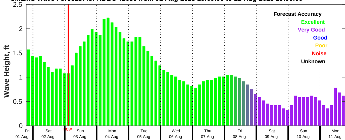
CMEMS Wave Forecast for NDBC 42036 from 01-Aug-2025 19:00:00 to 11-Aug-2025 19:00:00
