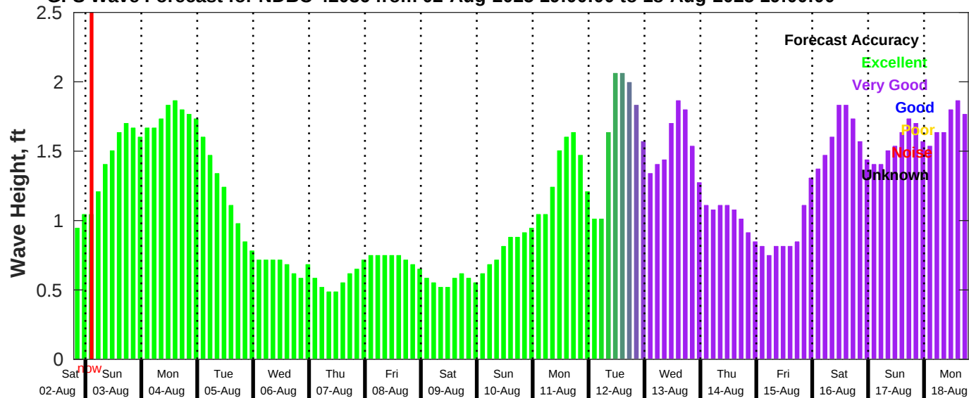
GFS Wave Forecast for NDBC 42036 from 02-Aug-2025 19:00:00 to 18-Aug-2025 19:00:00
