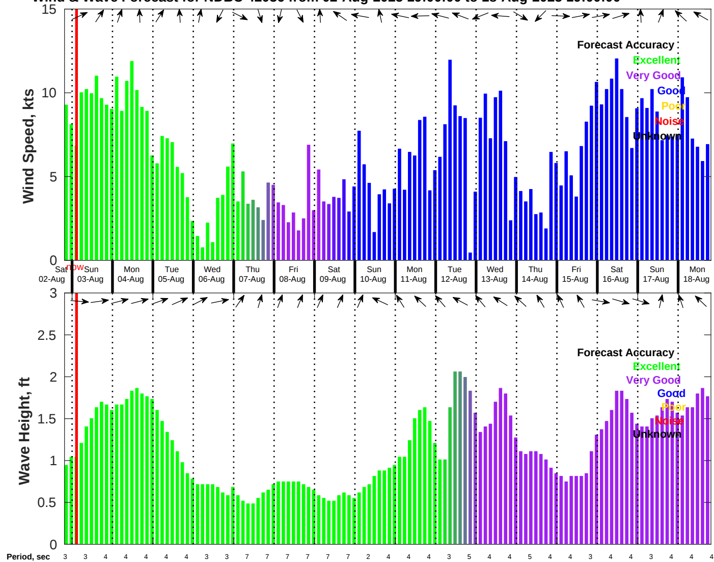
Wind & Wave Forecast for NDBC 42036 from 02-Aug-2025 19:00:00 to 18-Aug-2025 19:00:00
