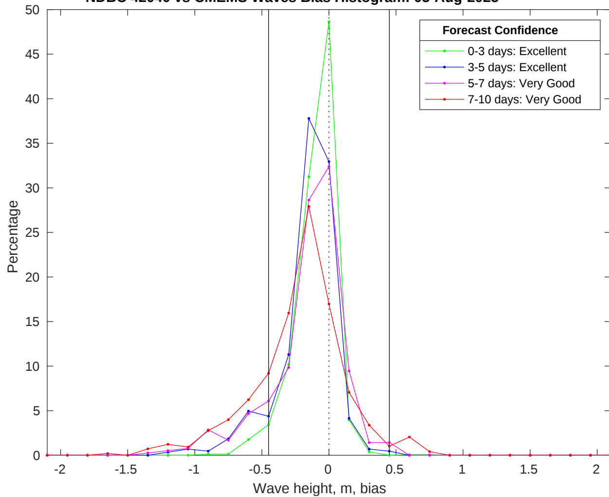
NDBC 42040 vs CMEMS Waves Bias Histogram: 03-Aug-2025
