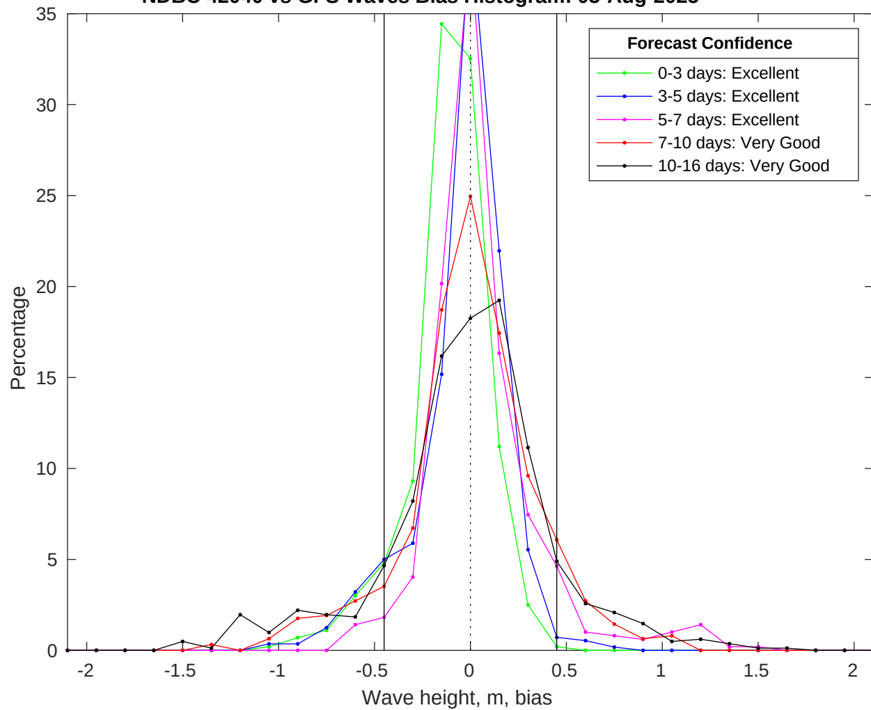
NDBC 42040 vs GFS Waves Bias Histogram: 03-Aug-2025
