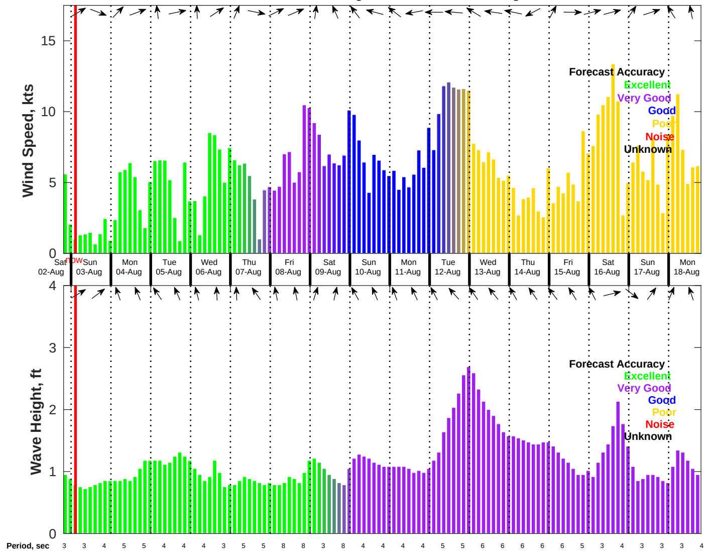
Wind & Wave Forecast for NDBC 42040 from 02-Aug-2025 19:00:00 to 18-Aug-2025 19:00:00
