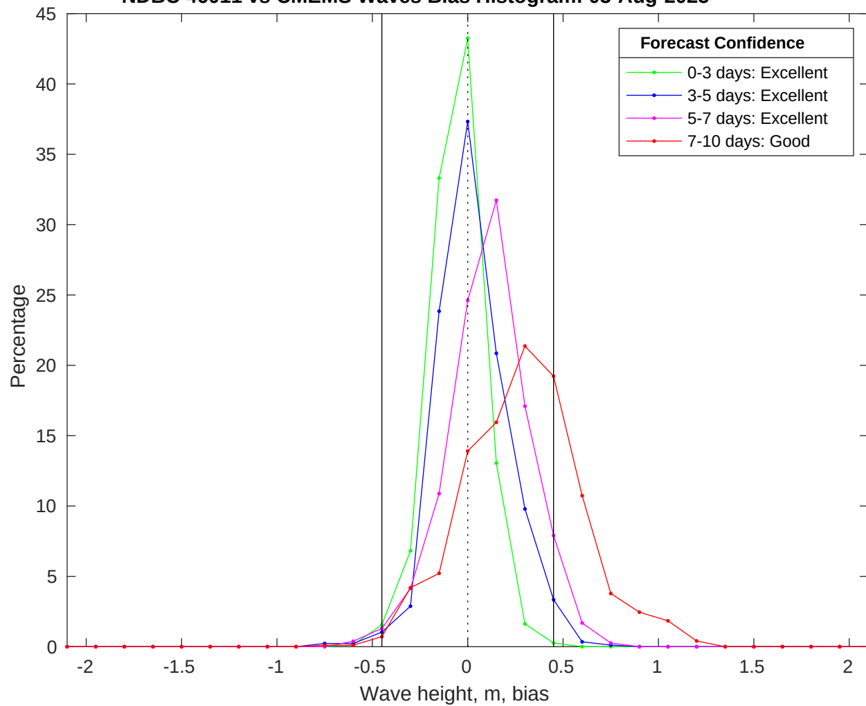
NDBC 46011 vs CMEMS Waves Bias Histogram: 03-Aug-2025
