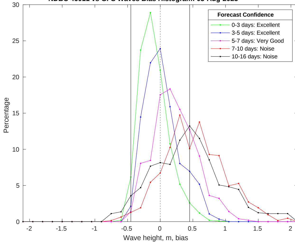
NDBC 46011 vs GFS Waves Bias Histogram: 03-Aug-2025
