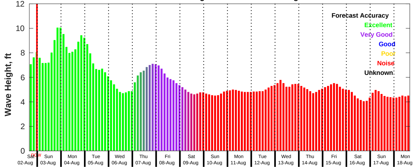
GFS Wave Forecast for NDBC 46011 from 02-Aug-2025 16:00:00 to 18-Aug-2025 16:00:00
