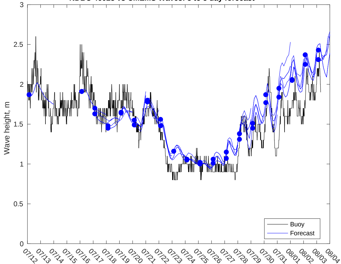
NDBC 46028 vs CMEMS Waves: 3 to 5 day forecast
