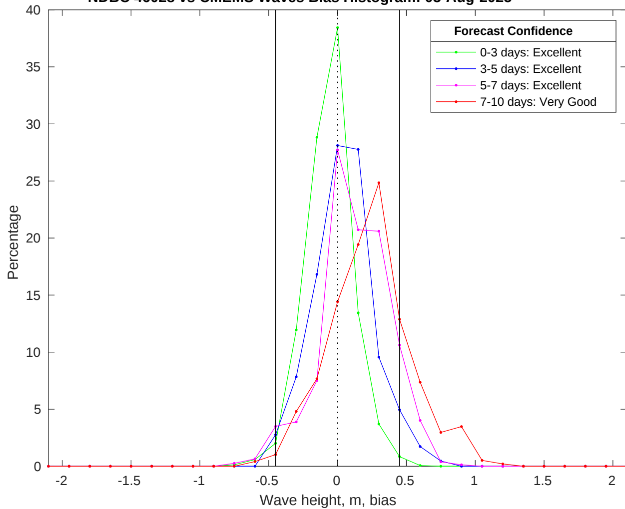
NDBC 46028 vs CMEMS Waves Bias Histogram: 03-Aug-2025
