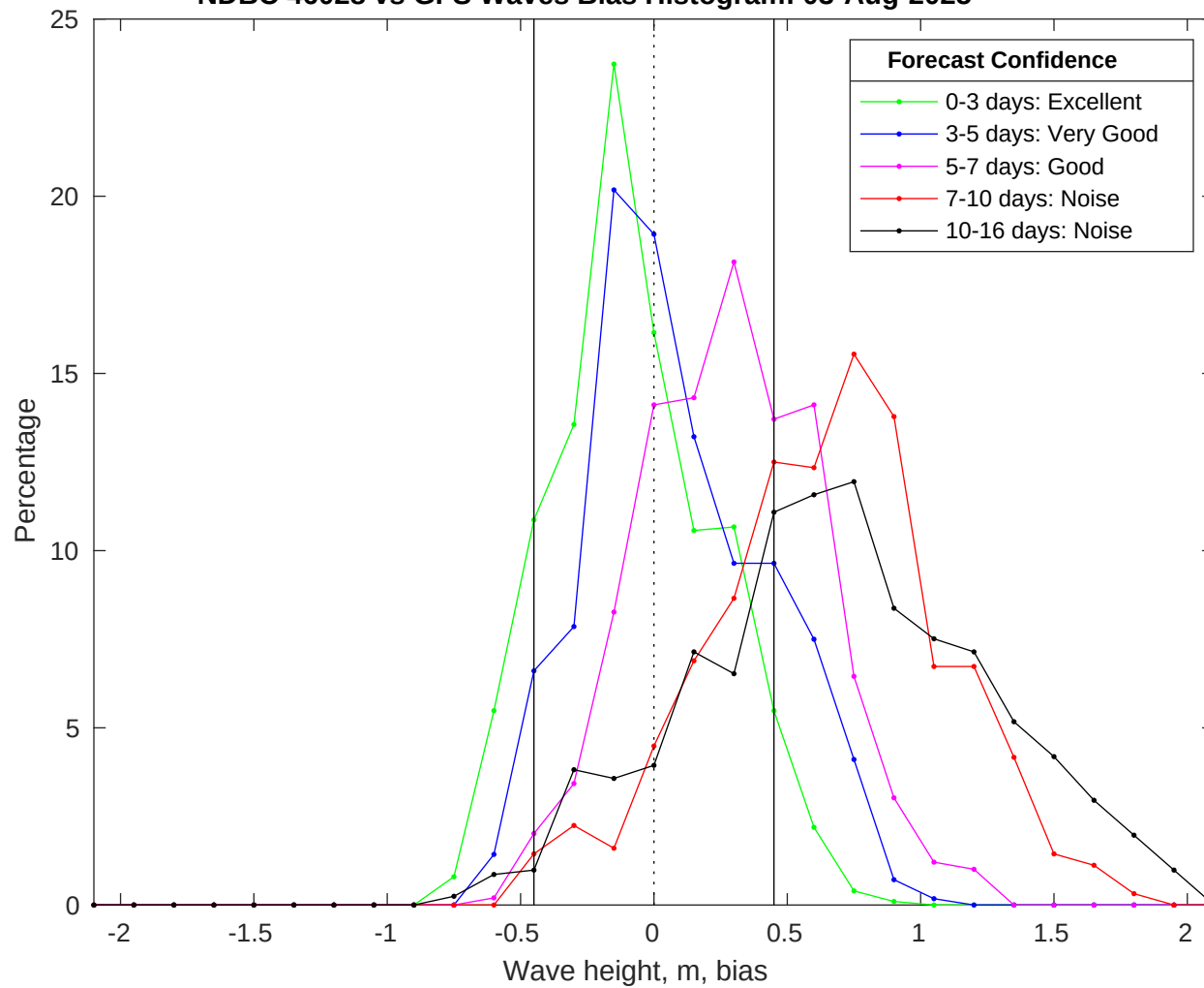
NDBC 46028 vs GFS Waves Bias Histogram: 03-Aug-2025
