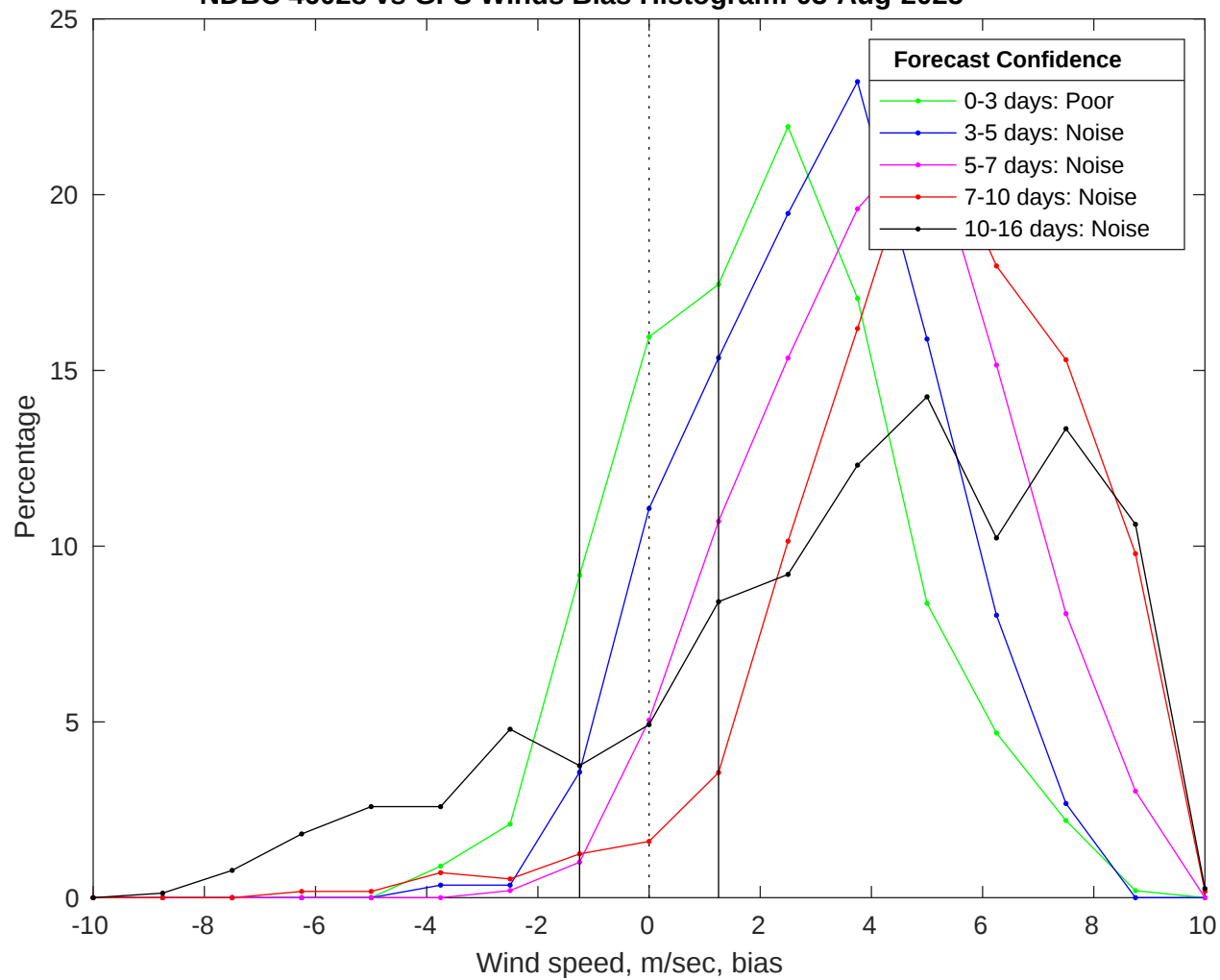
NDBC 46028 vs GFS Winds Bias Histogram: 03-Aug-2025
