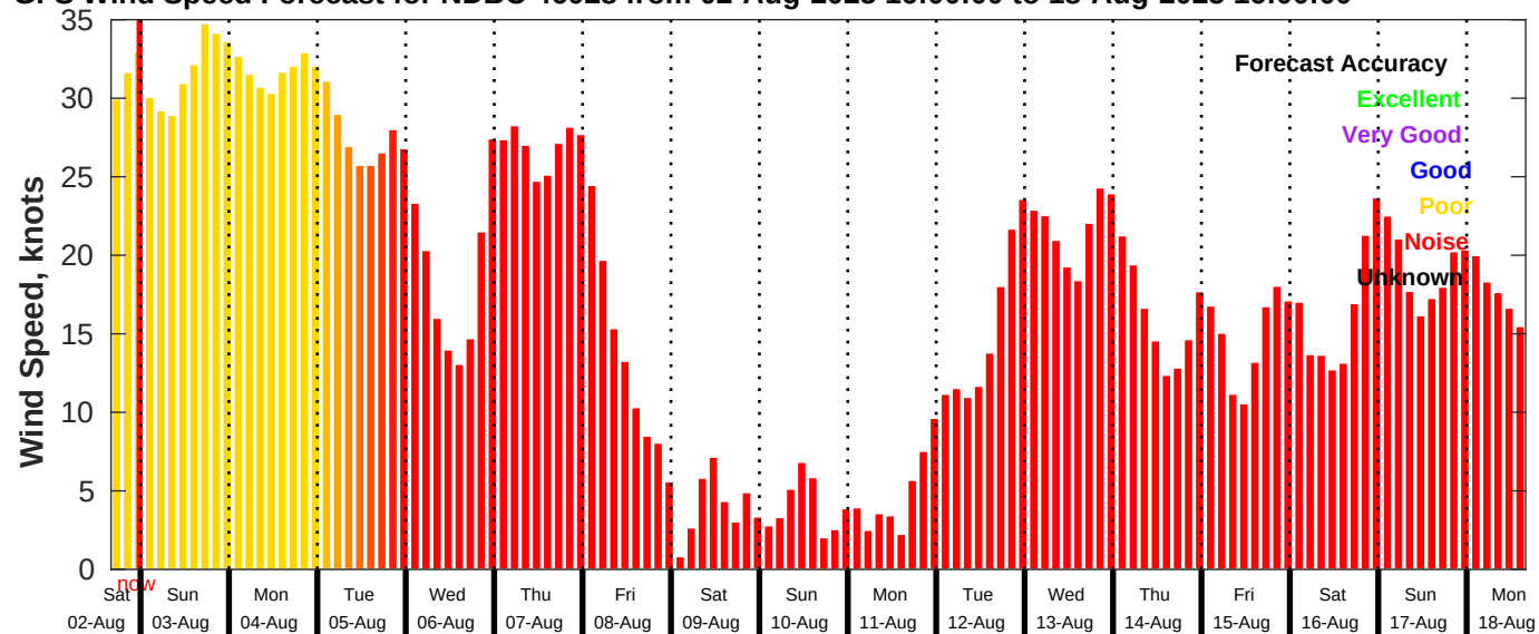
GFS Wind Speed Forecast for NDBC 46028 from 02-Aug-2025 16:00:00 to 18-Aug-2025 16:00:00
