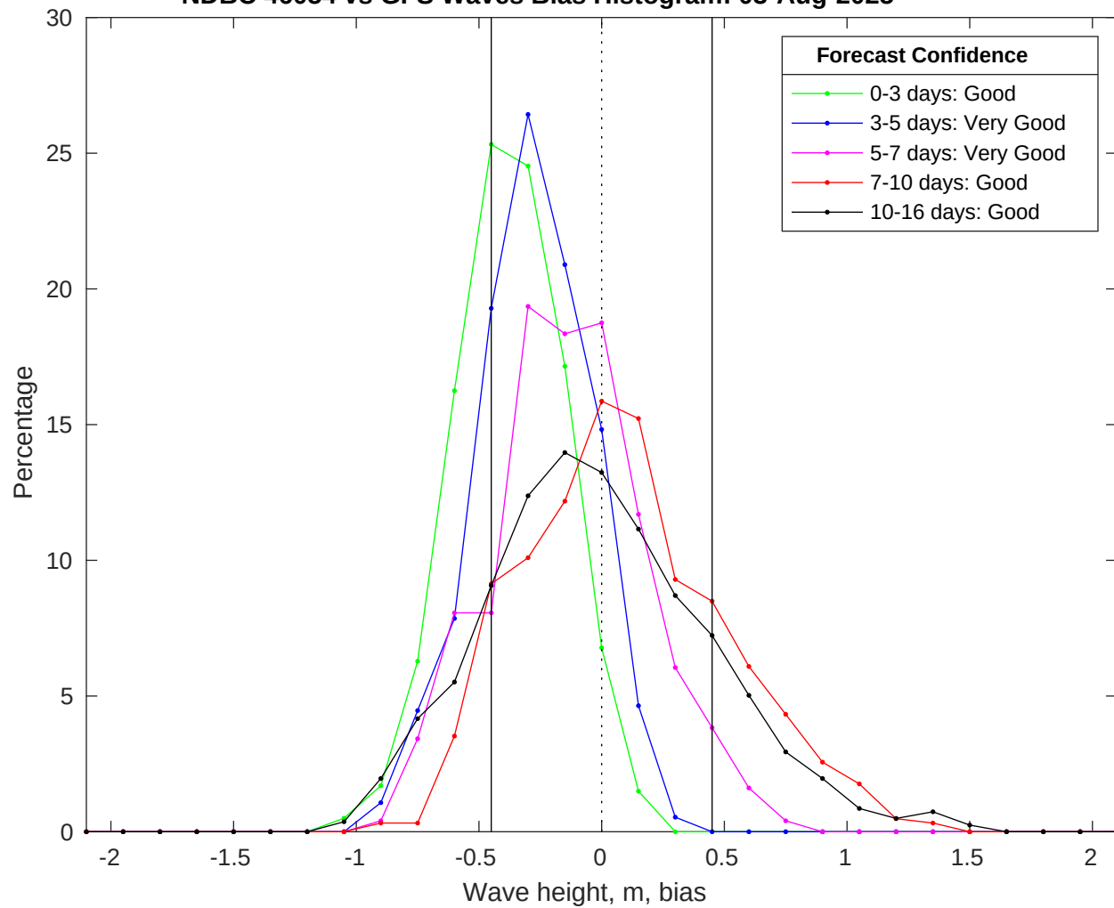
NDBC 46054 vs GFS Waves Bias Histogram: 03-Aug-2025
