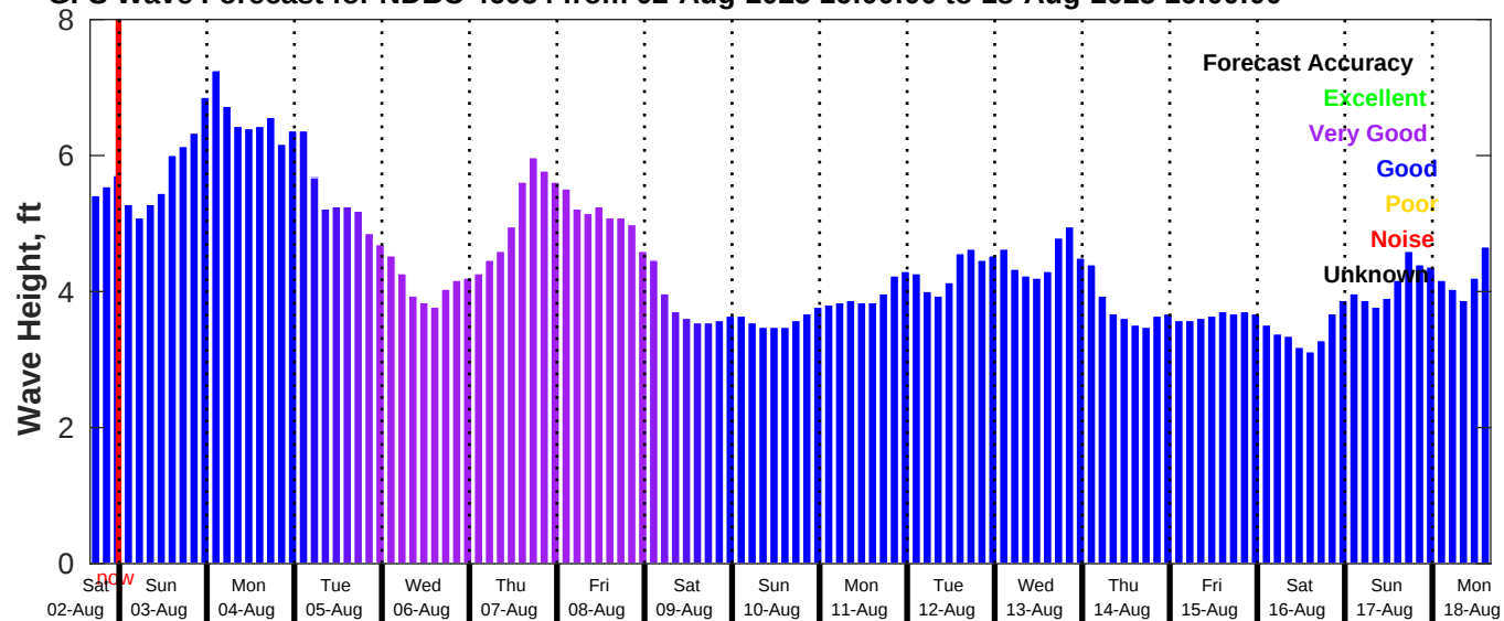
GFS Wave Forecast for NDBC 46054 from 02-Aug-2025 16:00:00 to 18-Aug-2025 16:00:00
