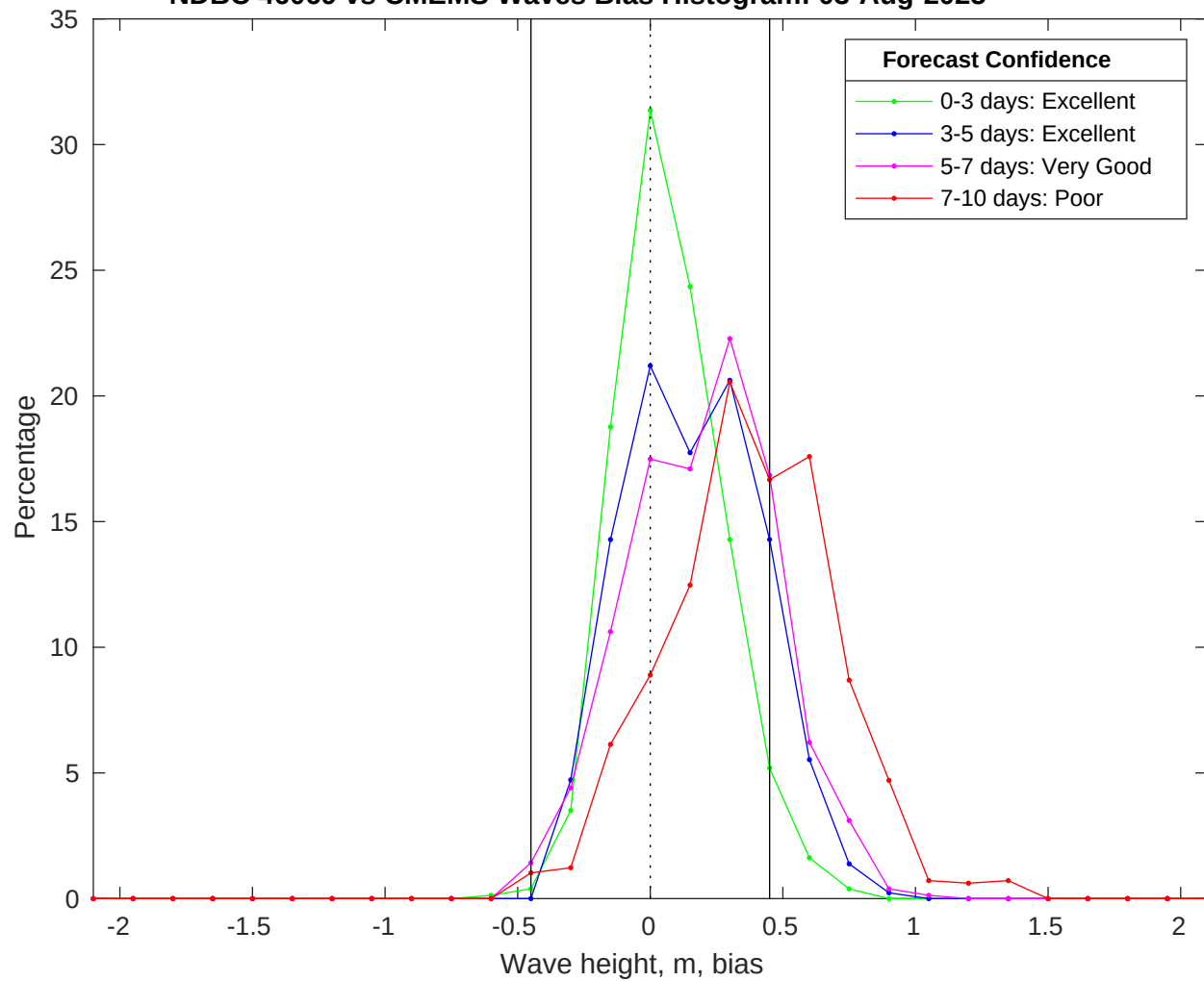
NDBC 46069 vs CMEMS Waves Bias Histogram: 03-Aug-2025
