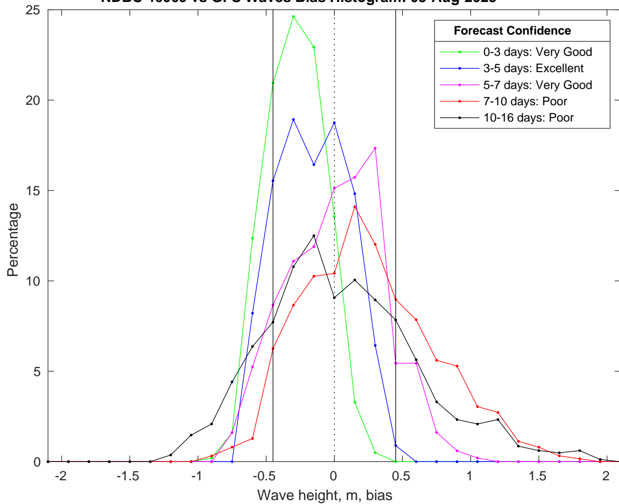
NDBC 46069 vs GFS Waves Bias Histogram: 03-Aug-2025
