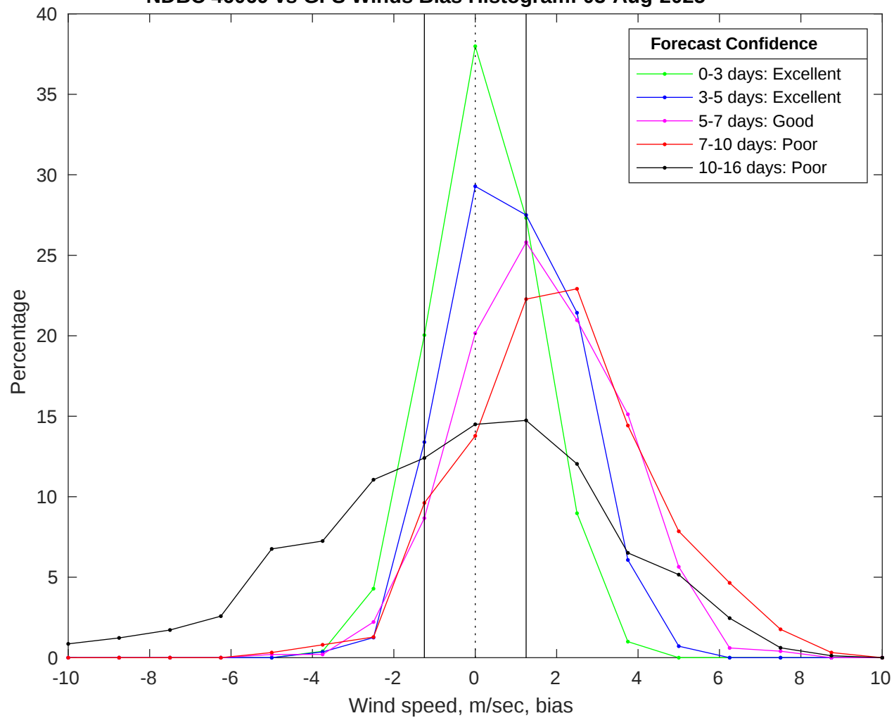
NDBC 46069 vs GFS Winds Bias Histogram: 03-Aug-2025
