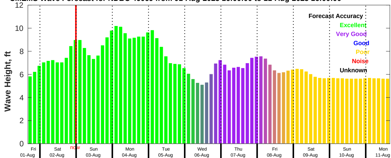
CMEMS Wave Forecast for NDBC 46069 from 01-Aug-2025 16:00:00 to 11-Aug-2025 16:00:00
