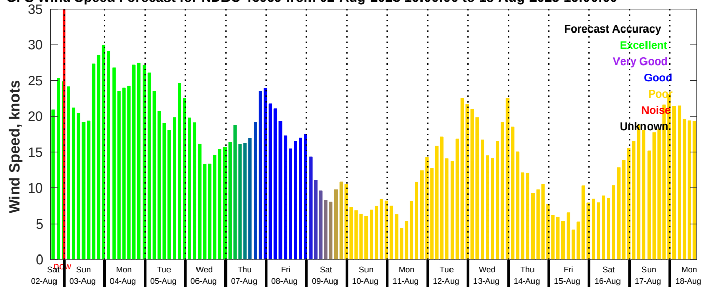
GFS Wind Speed Forecast for NDBC 46069 from 02-Aug-2025 16:00:00 to 18-Aug-2025 16:00:00
