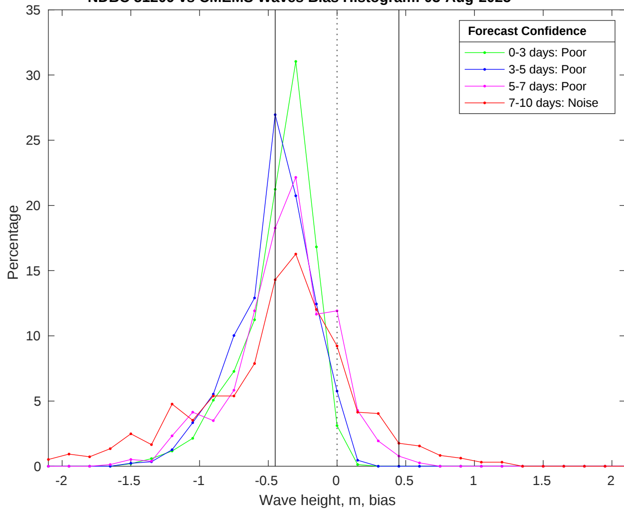
NDBC 51209 vs CMEMS Waves Bias Histogram: 03-Aug-2025
