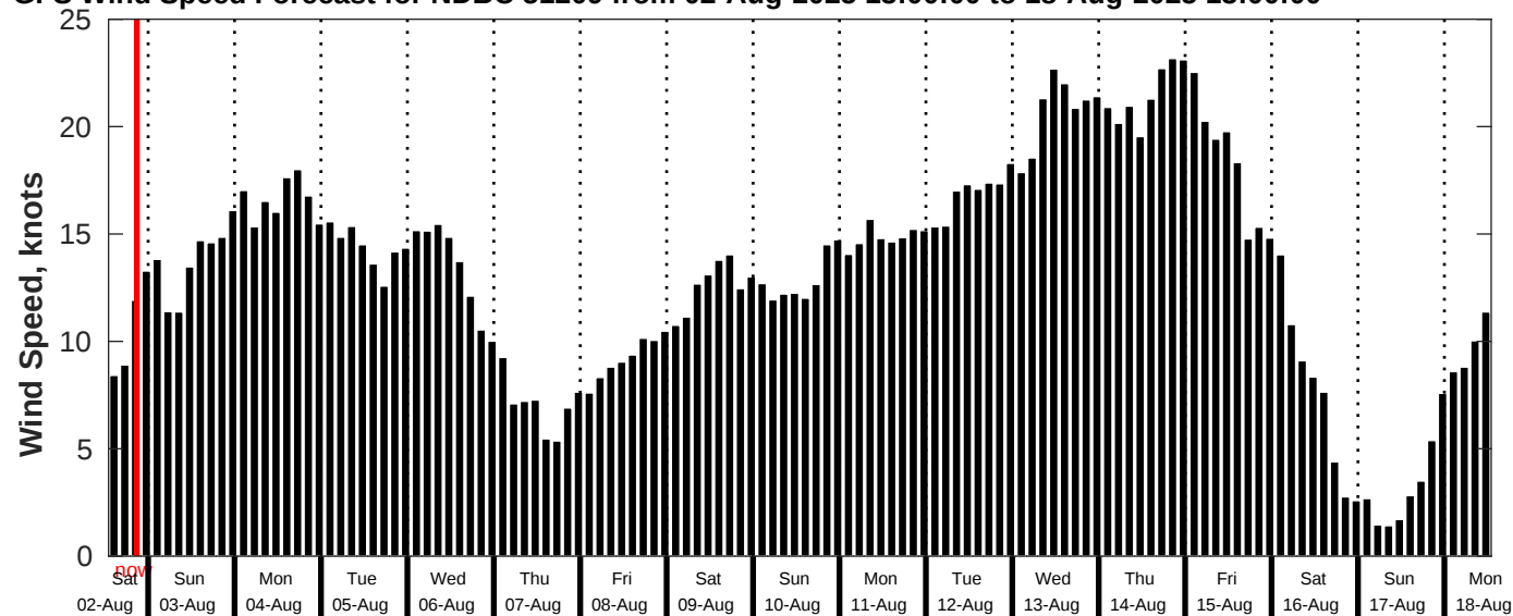
GFS Wind Speed Forecast for NDBC 51209 from 02-Aug-2025 13:00:00 to 18-Aug-2025 13:00:00
