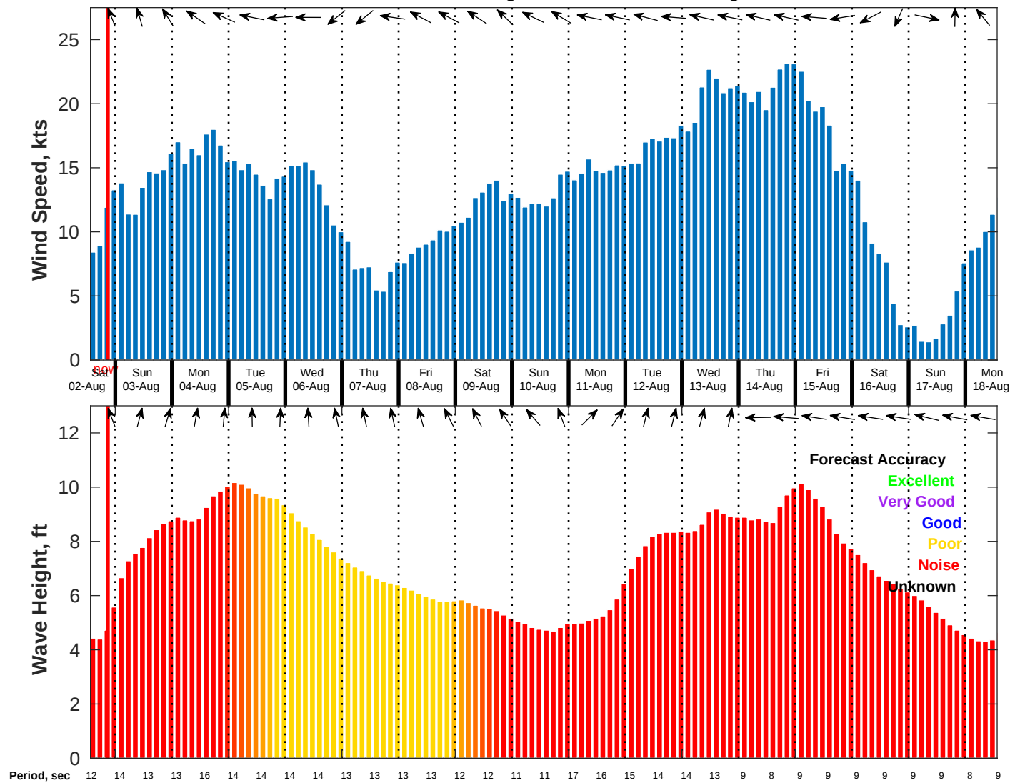
Wind & Wave Forecast for NDBC 51209 from 02-Aug-2025 13:00:00 to 18-Aug-2025 13:00:00
