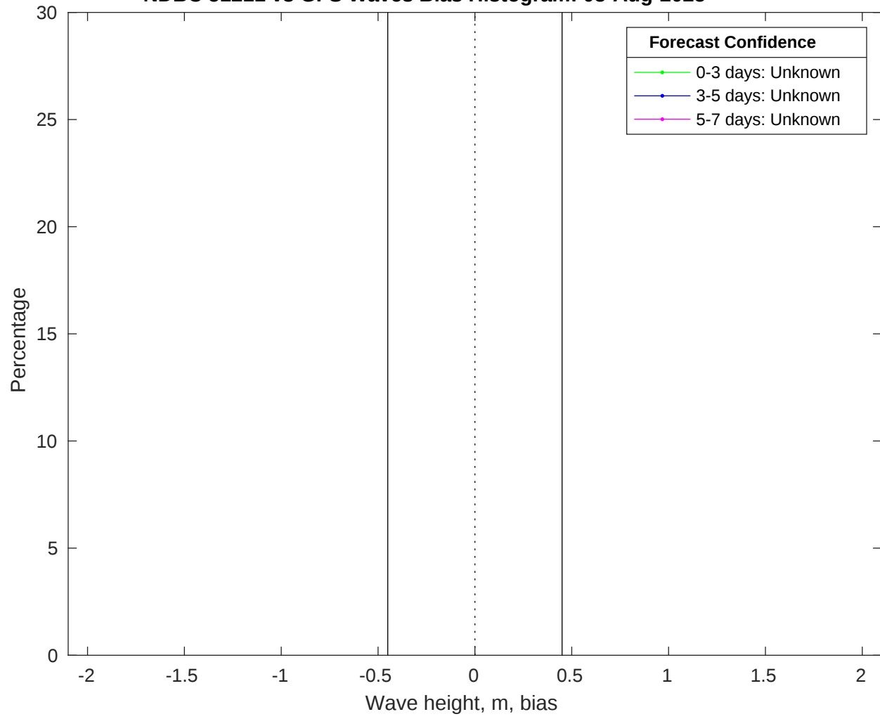
NDBC 51211 vs GFS Waves Bias Histogram: 03-Aug-2025
