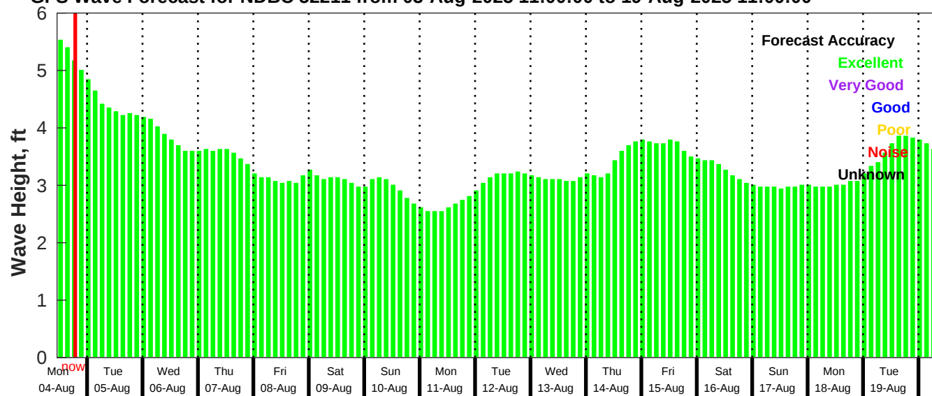
GFS Wave Forecast for NDBC 52211 from 03-Aug-2025 11:00:00 to 19-Aug-2025 11:00:00
